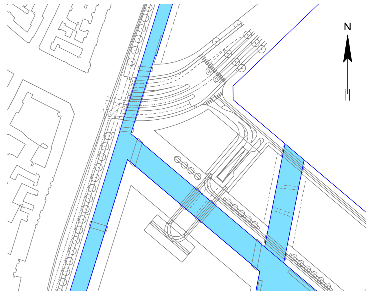
Plan of canal 1:2000
