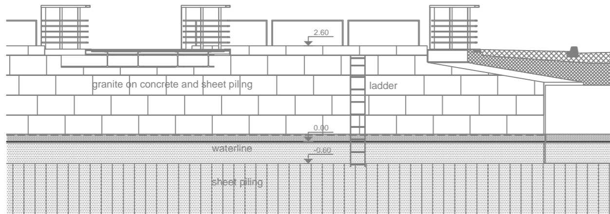
Part section of canal, granite 1:100
