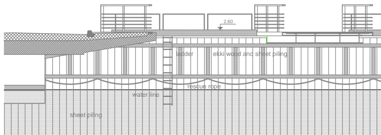
Part section of canal, ekki wood 1:100
